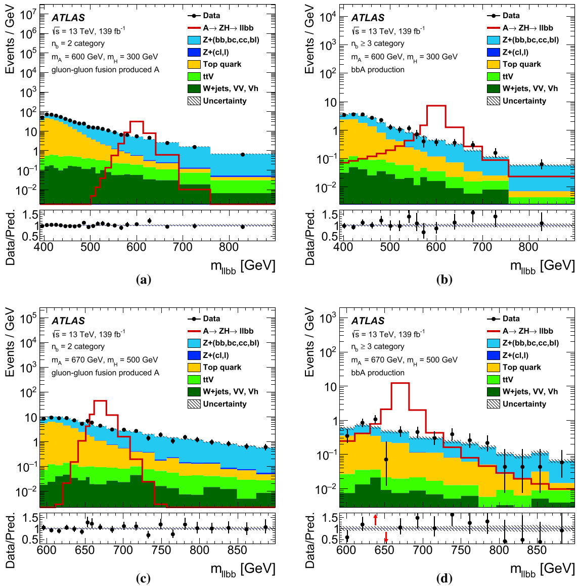
Fig. 8 The m_{\ell\ell b\bar{b}} mass distribution for the m_{bb} windows defined for m_H = 300 GeV and m_H = 500 GeV for a , c the n_b = 2 and b , d the n_b \geq 3 category, respectively. Signal distributions with (m_A, m_H) = (600, 300) GeV and (m_A, m_H) = (670, 500) GeV are
