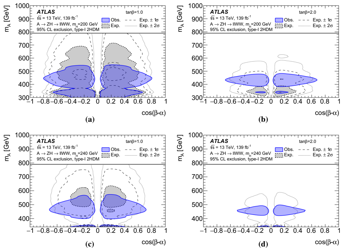
Fig. 14 Observed and expected 95% CL exclusion regions in the (\cos(\beta - \alpha), m_A) plane for various \tan \beta values for a , b m_H = 200 GeV and c , d m_H = 240 GeV in the context of type-I 2HDM for the \ell\ell WW channel
