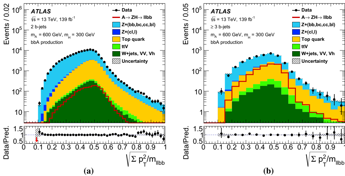
Fig. 2 The \sqrt{\Sigma p_T^2 / m_{\ell\ell bb}} distributions shown before the requirement on this variable is applied for events with a exactly two b -jets and b three or more b -jets. Corrections from a fit to the data are applied to the simulation, as described in Sects. 5.1 and 8. The signal distribution for (m_A, m_H) = (600, 300) GeV is also shown, and is normalised such that the production cross section times the branching ratios B(A \rightarrow ZH) and B(H \rightarrow bb) corresponds to 1 pb. The signal shown includes only A bosons produced in association with b -quarks. The lower panel shows the ratio of the data to the background prediction (black filled circles) and the relative uncertainty,
